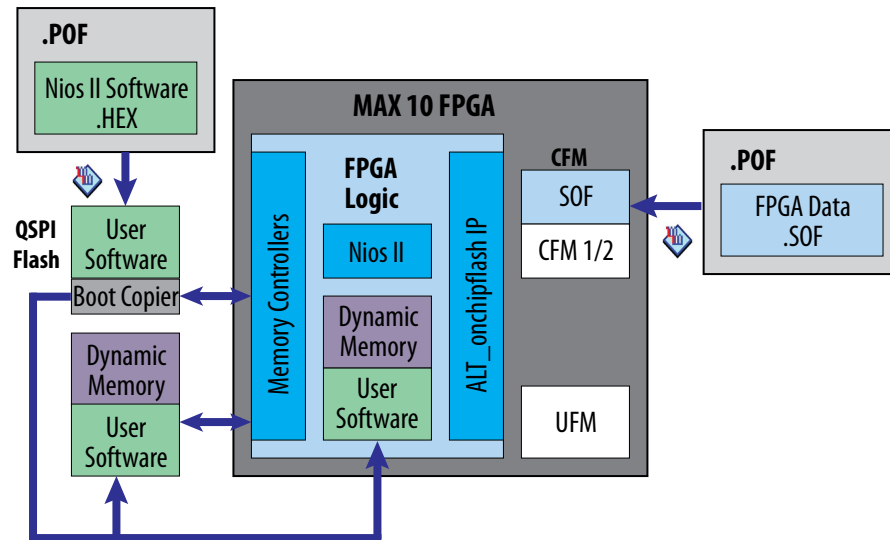
Figure 131. Block Diagram
