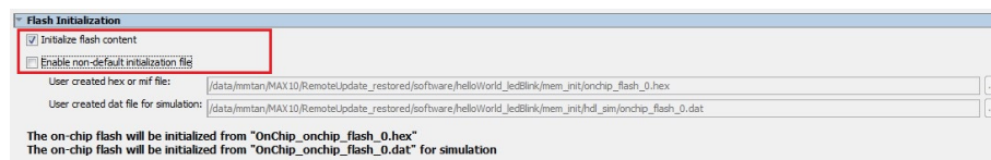
Figure 75. Initialize Flash Contents with Default Initialization File
