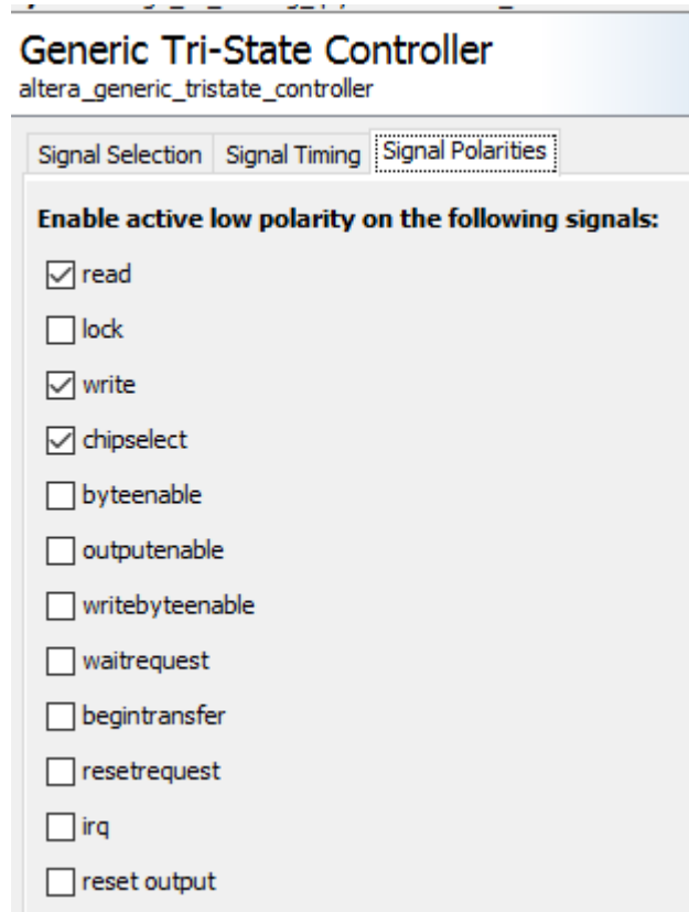
Figure 194. Signal Polarities
