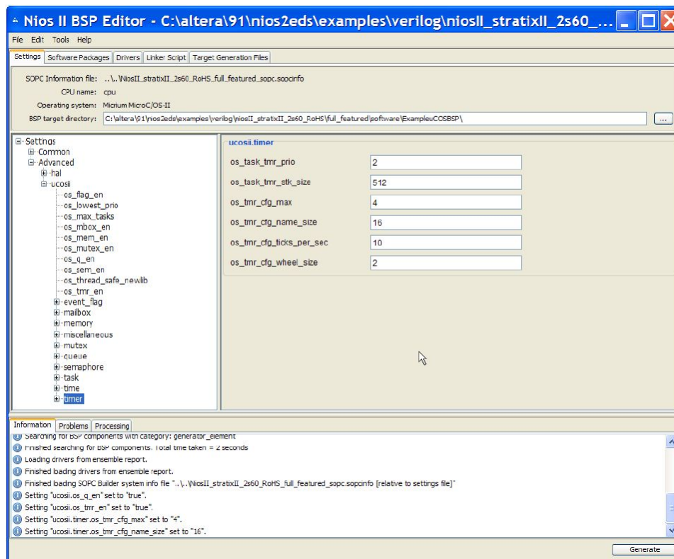
Figure 34. Configuring MicroC/OS-II for Four Timers in BSP Editor
