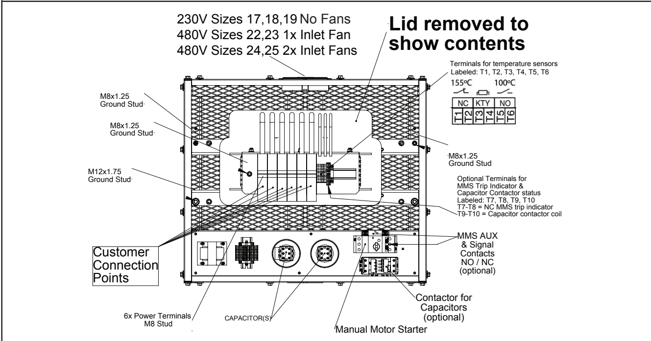
Figure 2.5.4 - Top View - dimensions mm [in]
