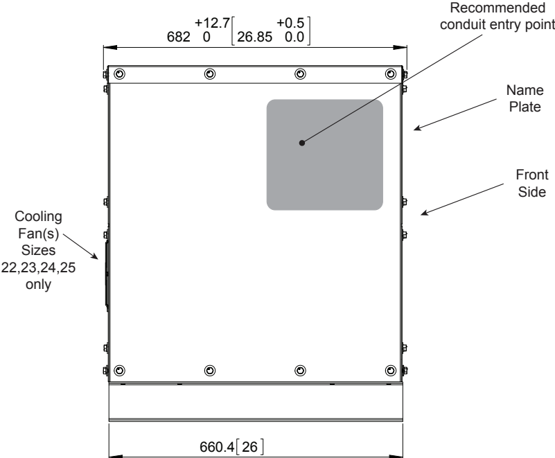
Figure 2.5.2 - Side View - dimensions mm [in]
