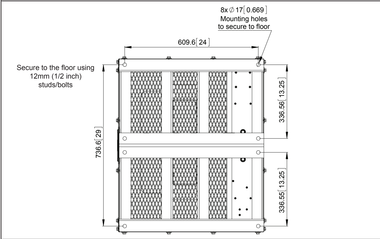
Figure 2.5.3 - Bottom View - dimensions mm [in]
