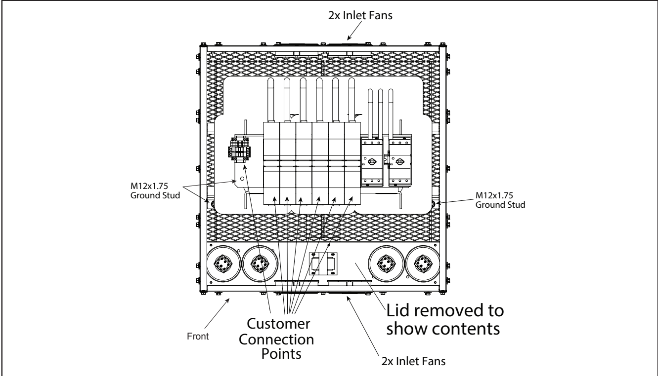
Figure 2.5.8 - Top View - dimensions mm [in]
