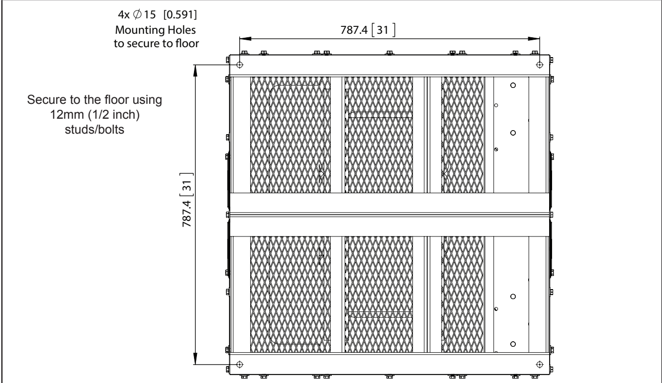
Figure 2.5.7 - Bottom View - dimensions mm [in]
