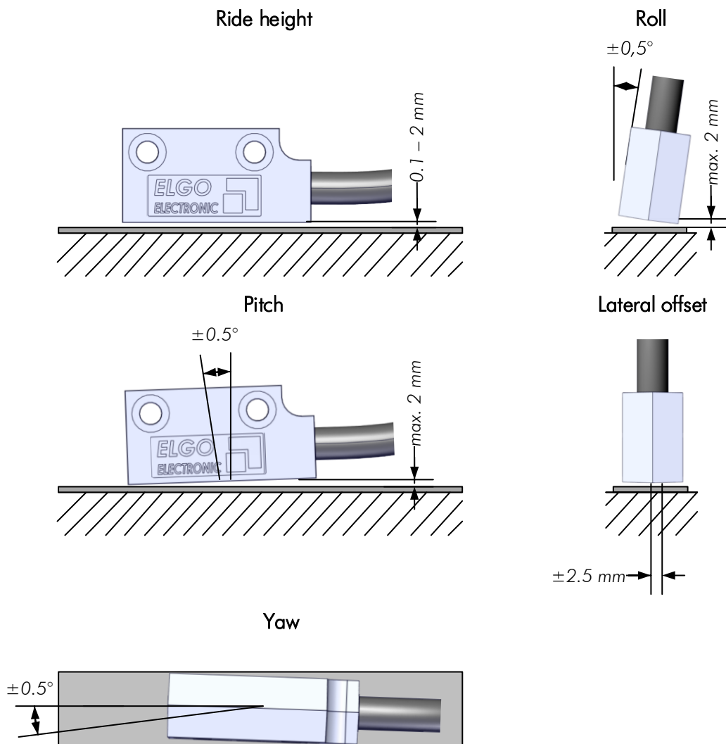
Figure 6: Sensor mounting tolerances
