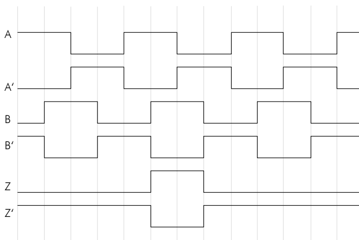
Figure 2: Pulse Diagram
