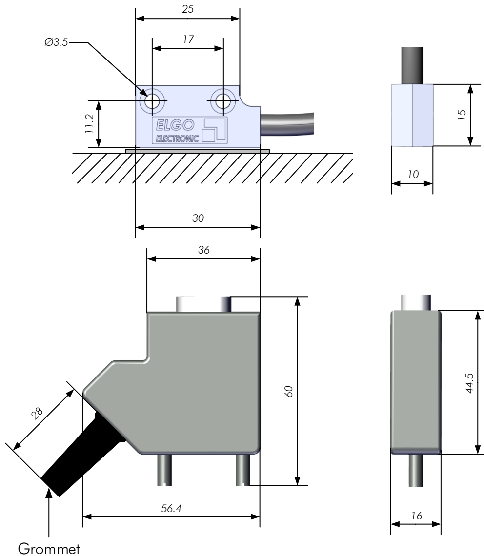
Figure 3: Dimensions Sensor and D-SUB Connector
